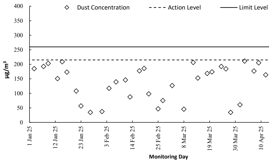
Graphical Plot for 24-Hour TSP Monitoring Result at AM(D)7a
